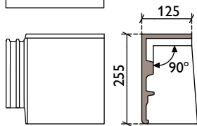
chaperongevelpan links
